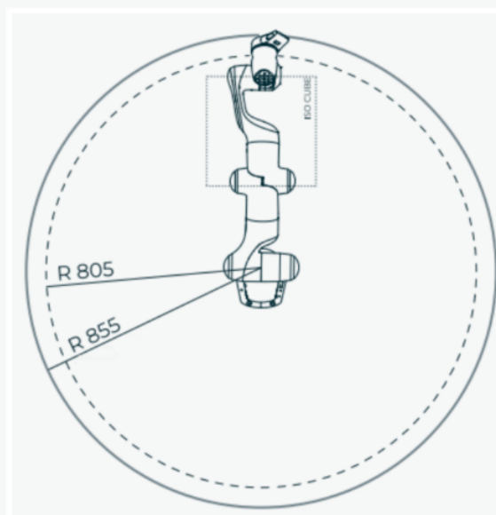
Top view of workspace 1 [mm]
