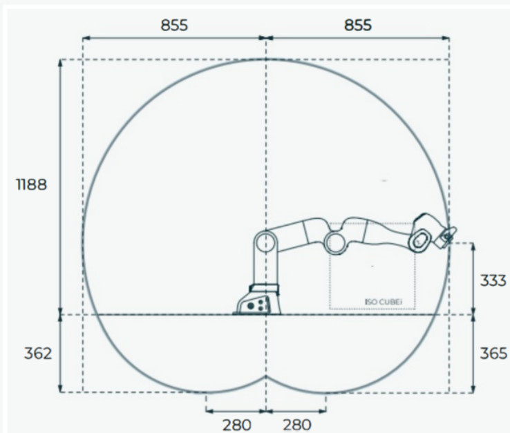
Side view of workspace 1 [mm]
