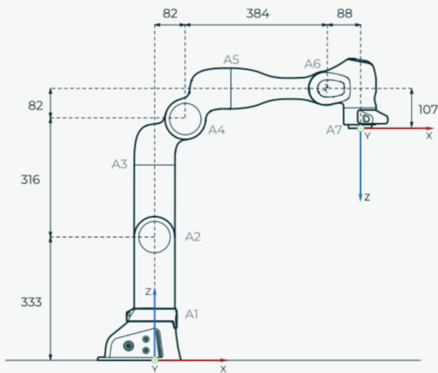
Shaft name and connecting rod distance [mm]
