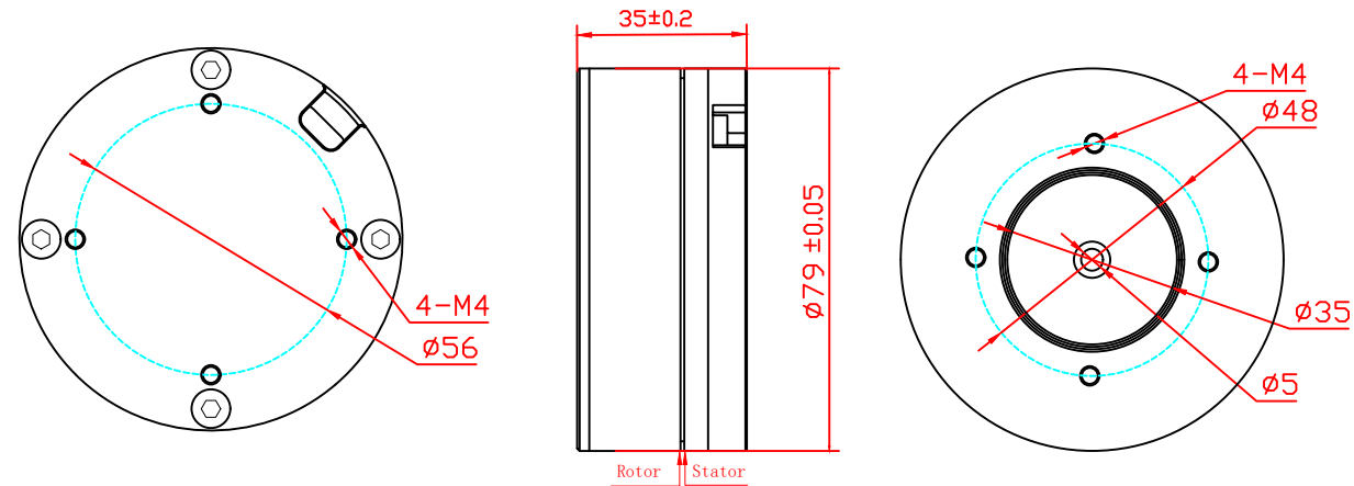
with encoder housing
