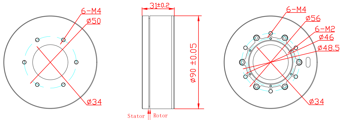
without encoder housing
