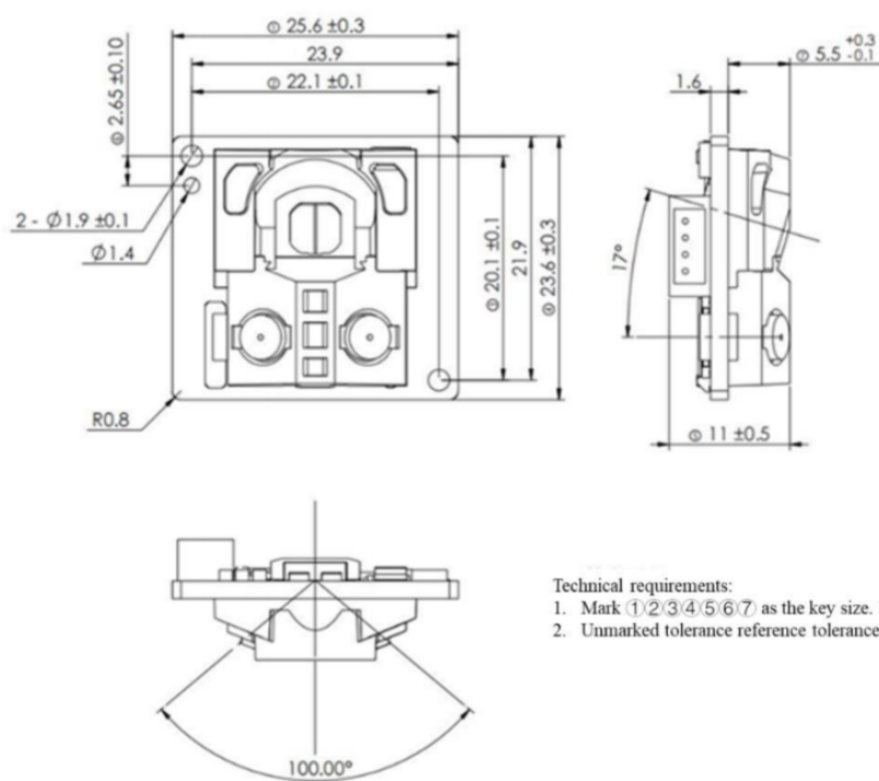
FIG 1A YDLIDAR GS2-S808G01 INSTALLATION&MECHANICAL SIZE (SCREW SPECIFICATIONS: PB1.7MM)
