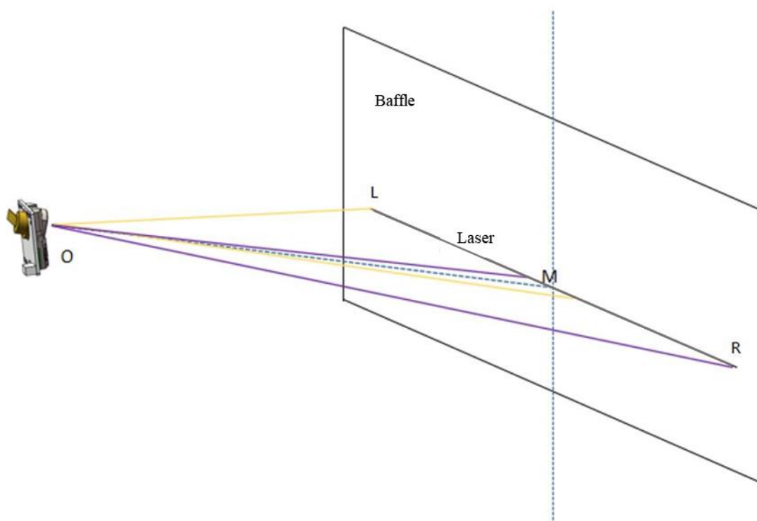
FIG 1 YDLIDAR GS5 MEASUREMENT DIAGRAM
