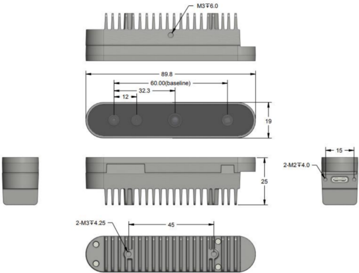
FIG 4 STRUCTURAL DRAWINGS
