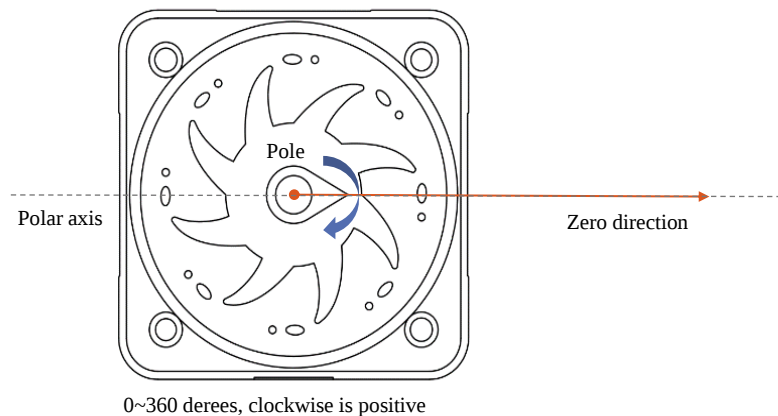
FIG 4 YDLIDAR T-MINI PLUS POLAR COORDINATE SYSTEM DEFINITION
