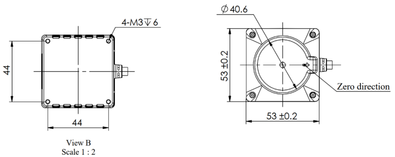
FIG 1 YDLIDAR TEA INSTALLATION DIMENSION (UNIT:MM)
