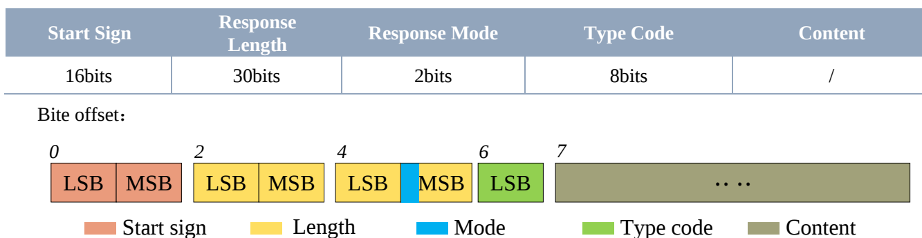
FIG 3 YDLIDAR TG SERIES SYSTEM MESSAGE DATA PROTOCOL
