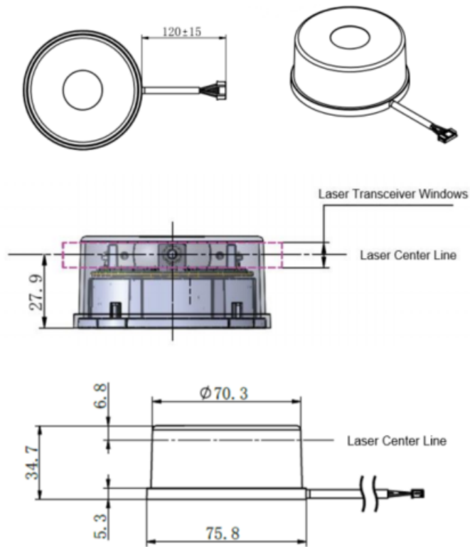
FIG 1 YDLIDAR TG5 INSTALLATION SIZE (UNIT: MM)
