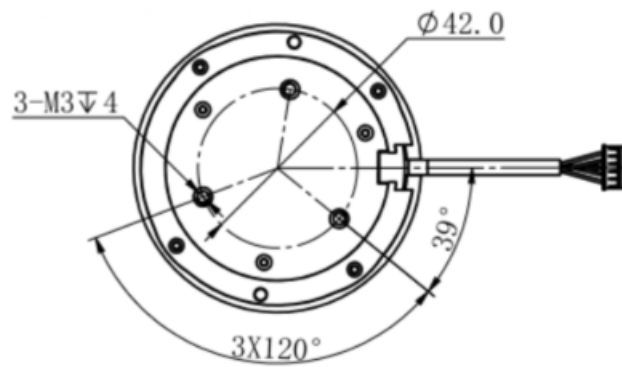
FIG 1 YDLIDAR TG5 INSTALLATION SIZE (UNIT: MM)
