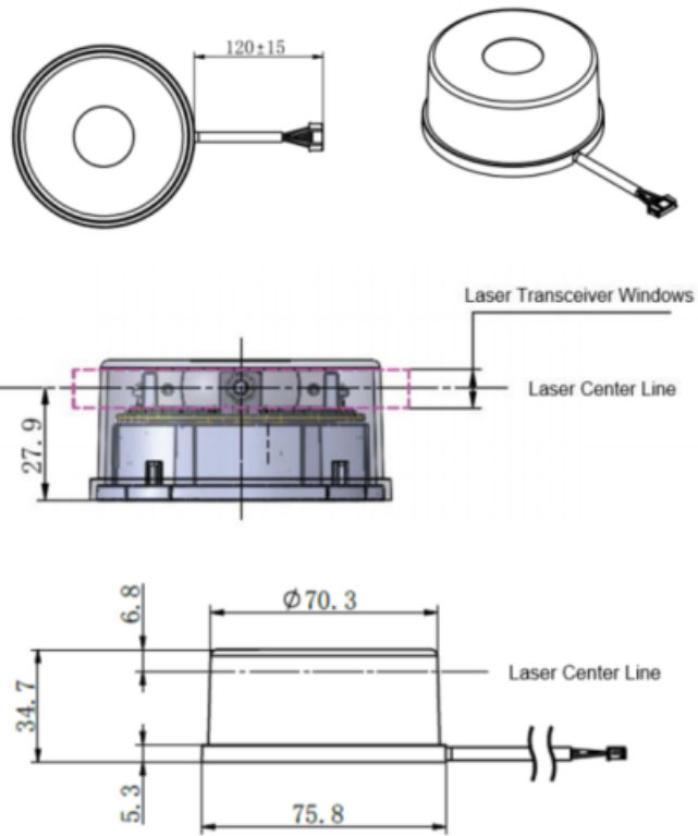
FIG 1 YDLIDAR TG30 INSTALLATION SIZE (UNIT: MM)
