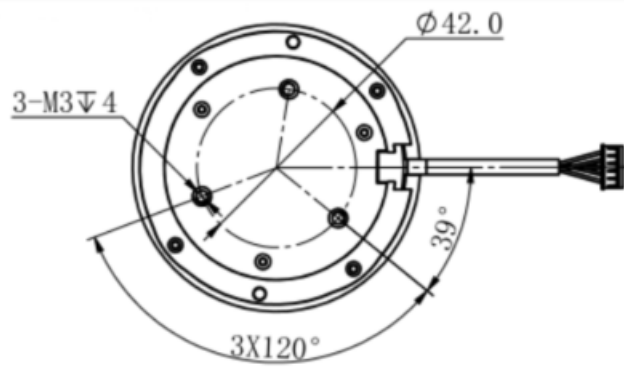
FIG 1 YDLIDAR TG30 INSTALLATION SIZE (UNIT: MM)
