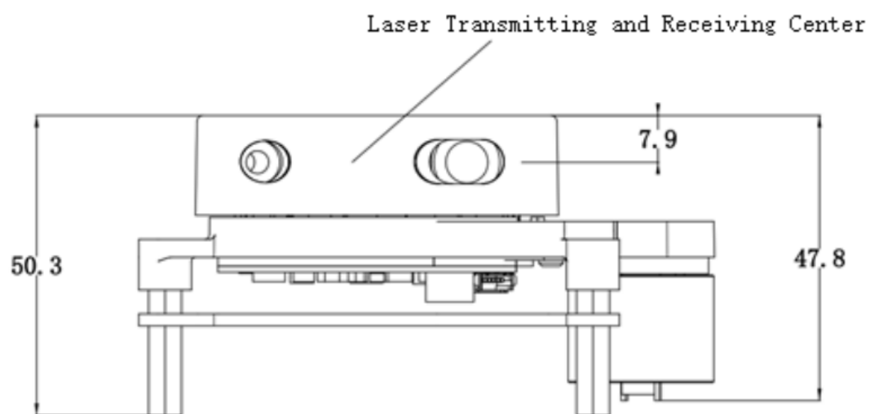
FIG 1 YDLIDAR X2 FRONT STRUCTURE SIZE (UNIT:MM)
