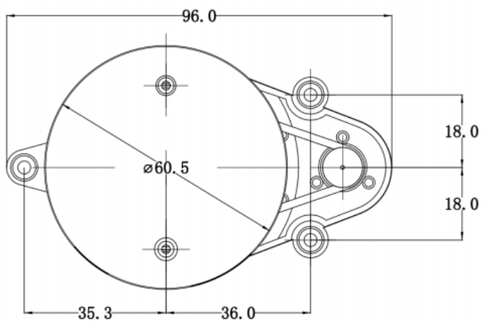
FIG 2 YDLIDAR X2 MECHANICAL DIMENSIONS (UNIT:MM)
