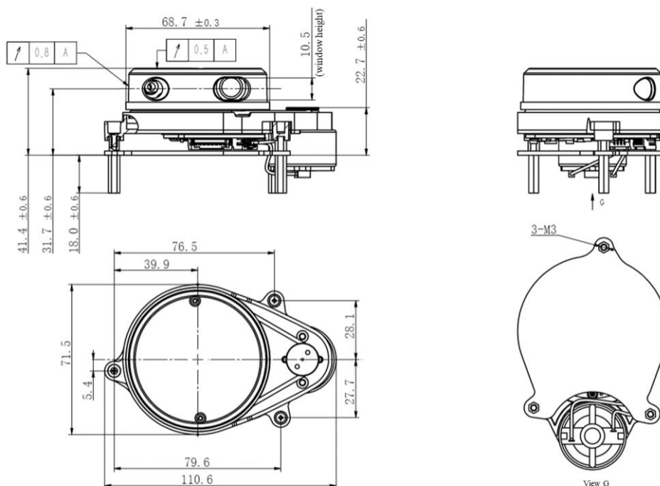
FIG 1 YDLIDAR X4PRO MECHANICAL DIMENSIONS (UNIT: MM)
