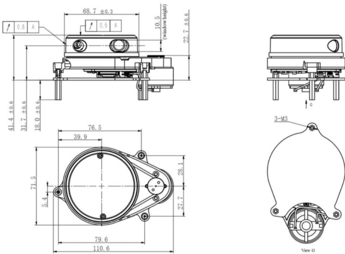
FIG 1 YDLIDAR X4PRO MECHANICAL DIMENSIONS (UNIT: MM)
